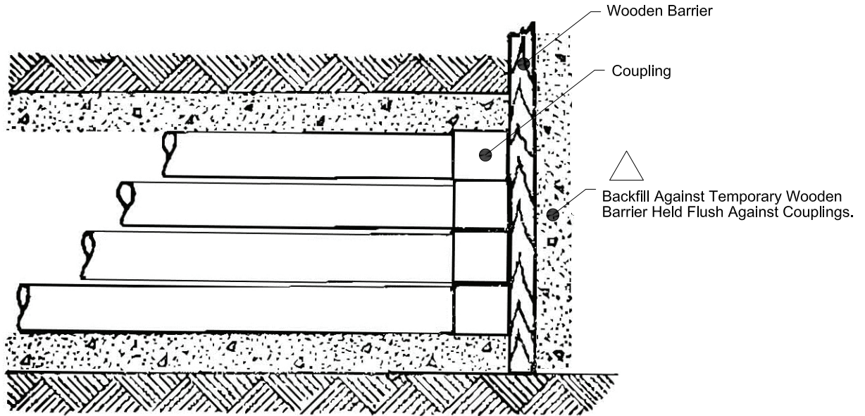
Typical Duct Bank
