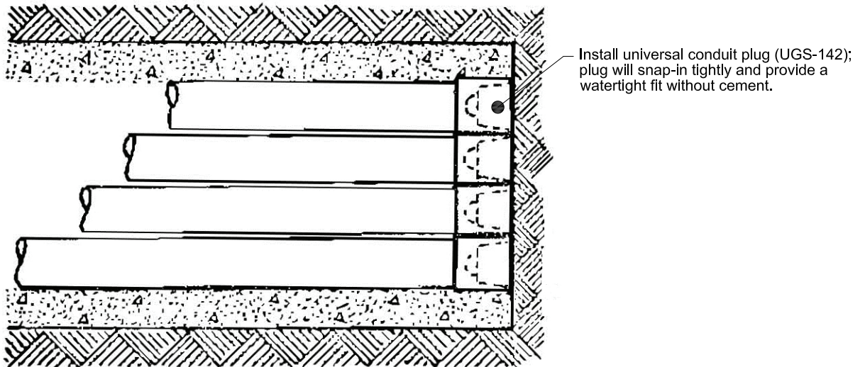
Completely Capped Duct Assembly
